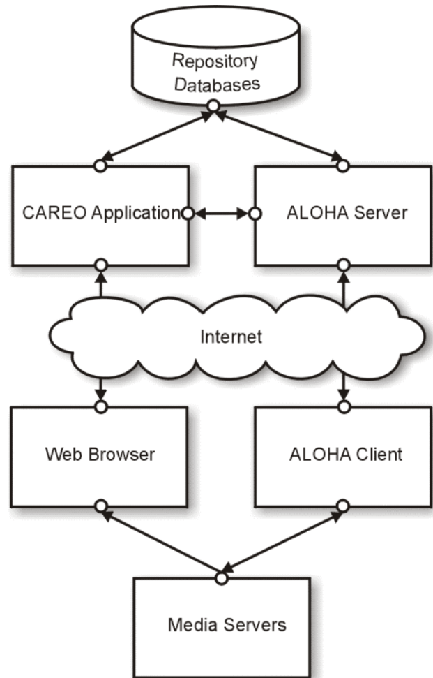
Figure 1. CAREO/ ALOHA Architecture
