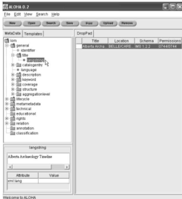
Figure 2. ALOHA Interface
