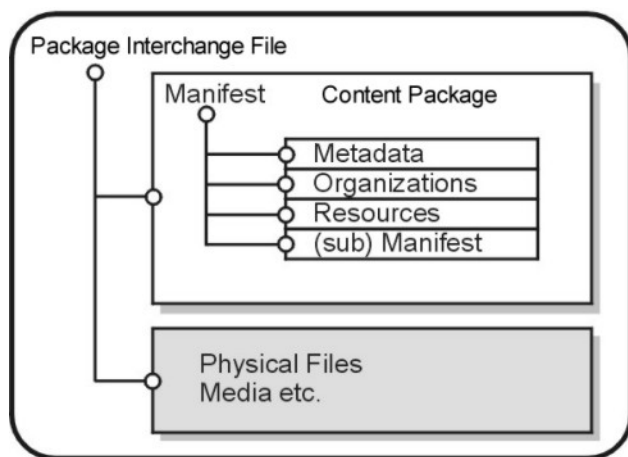
Figure 3. IMS Package Interchange File
